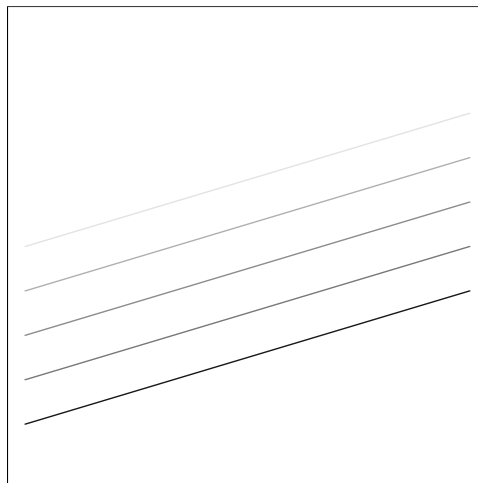
Figure 1: Varying Intercepts
