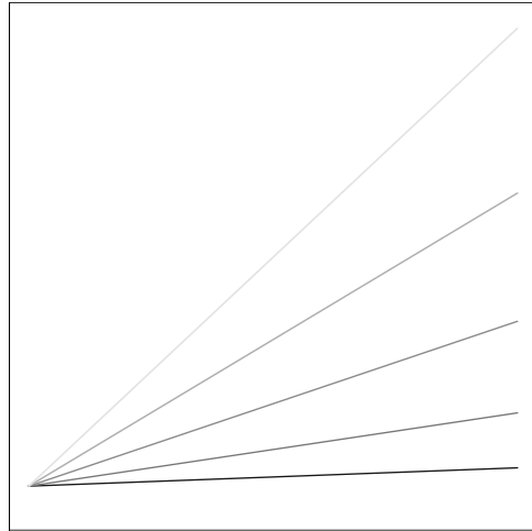
Figure 2: Varying Slopes
